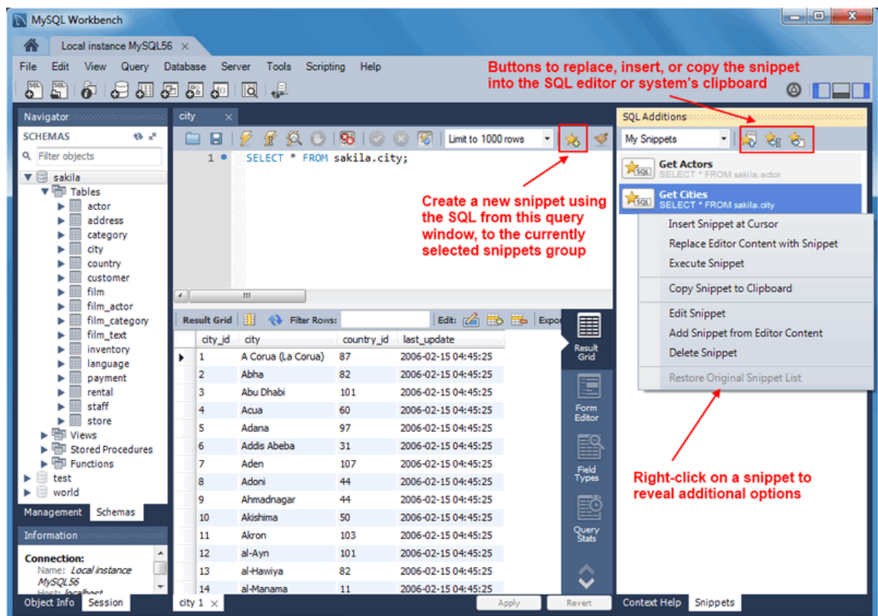
Figure 7.5 SQL Snippets: Usage
