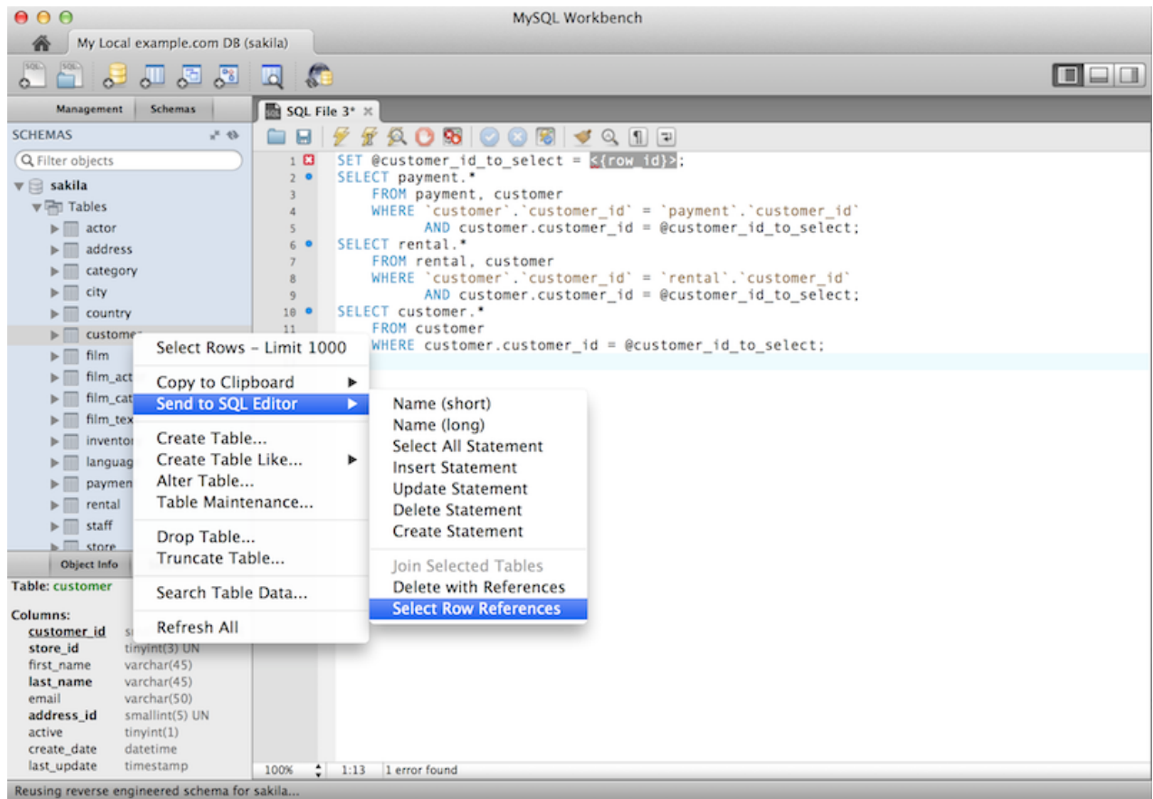
Figure 1.35 Cascading SELECT
