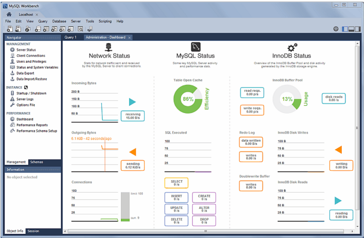
Figure 6.1 Performance: Dashboard
