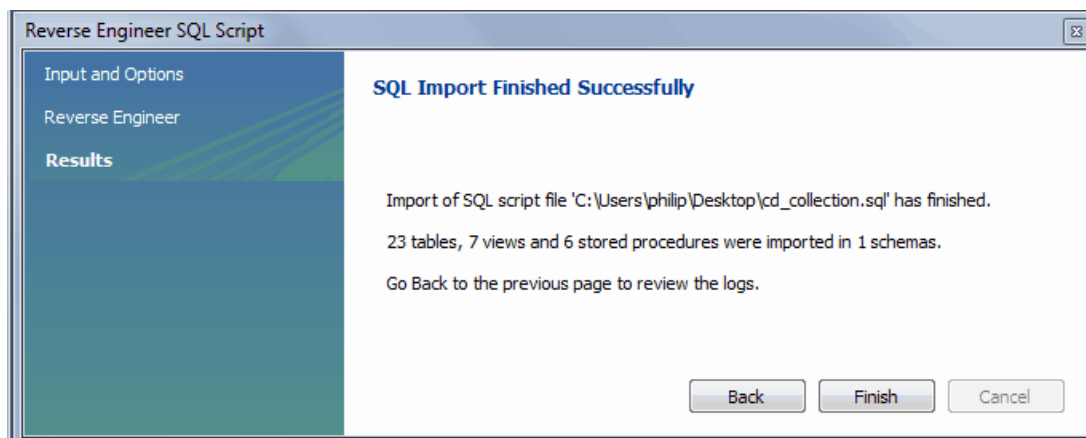
Figure 8.38 Review Script
