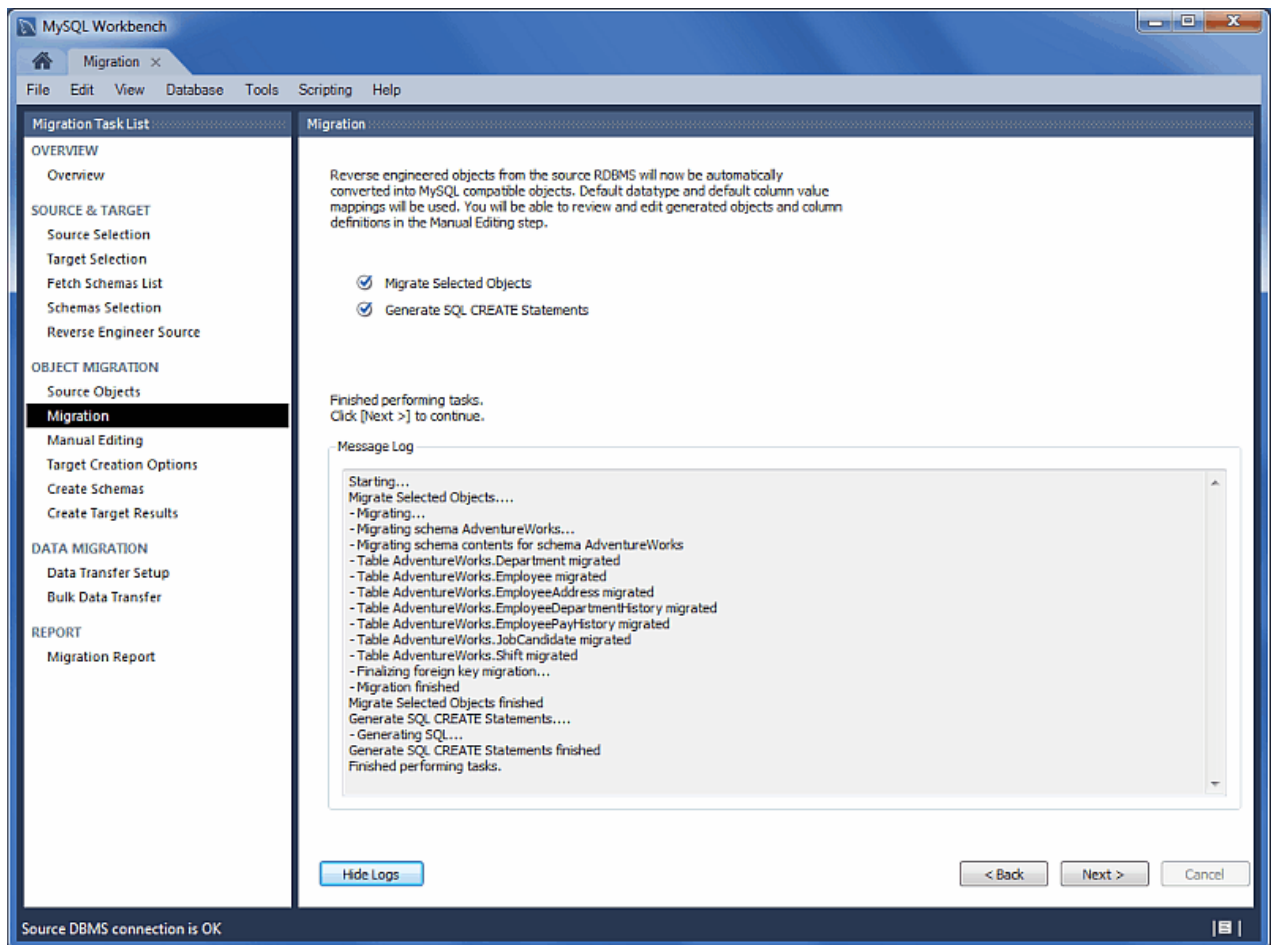
Figure 9.10 MySQL Workbench migration: Migration
