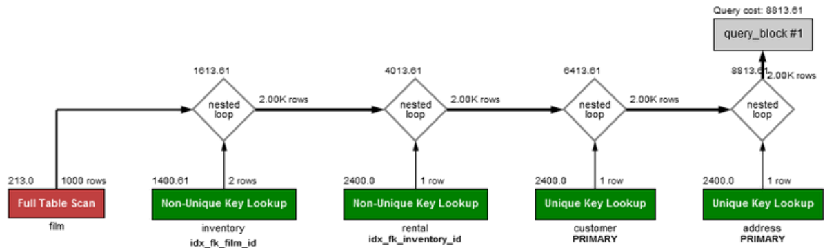
Figure 6.5 A Visual Explain Example
