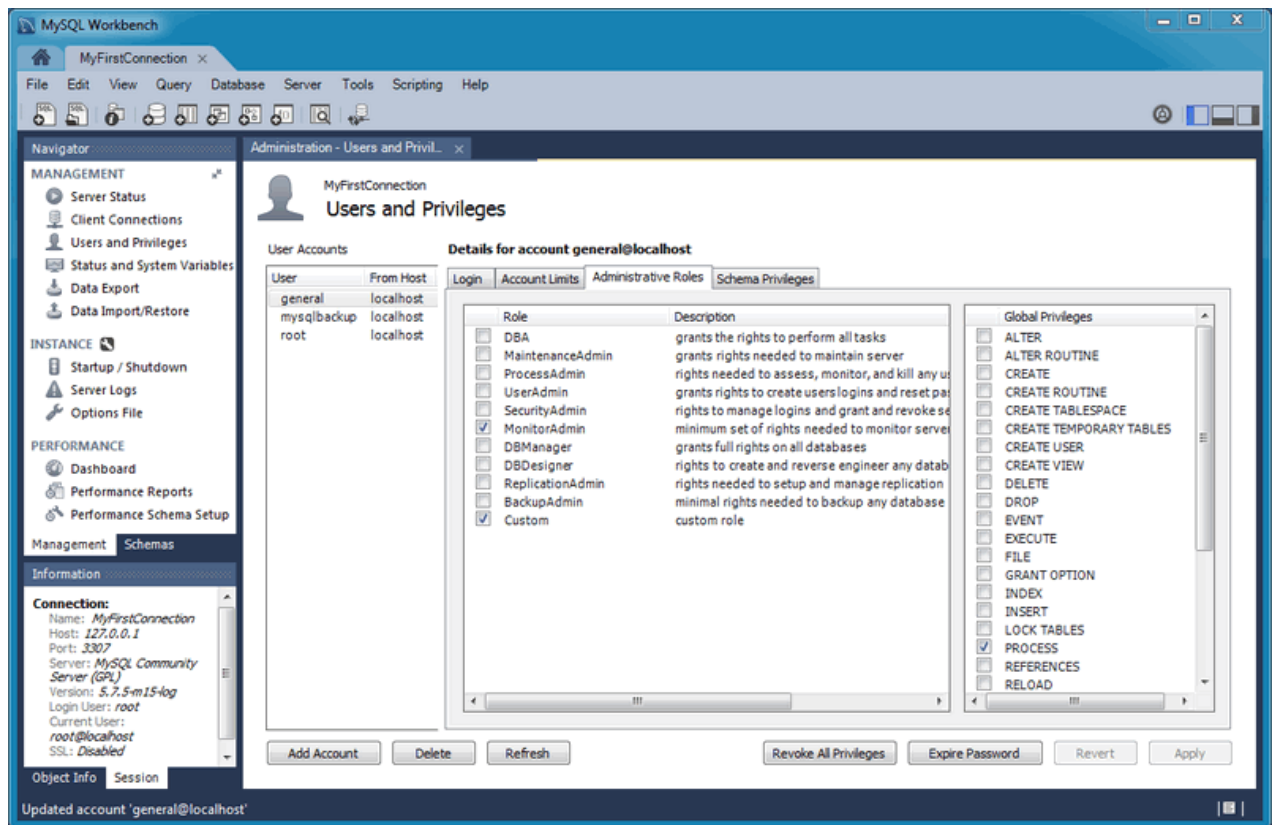
Figure 5.34 Navigator Management: User And Privileges: Administrative Roles
