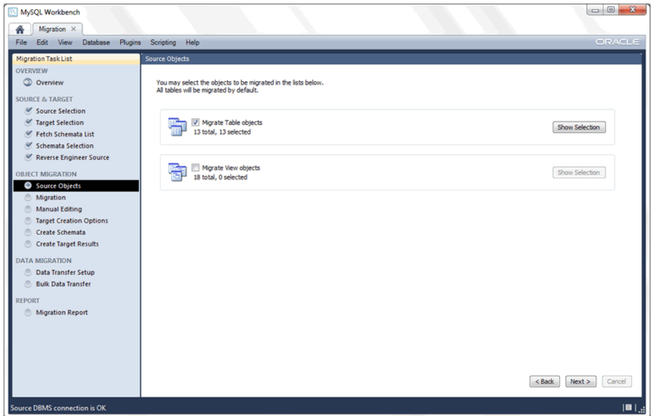
Figure 9.30 Source Objects
