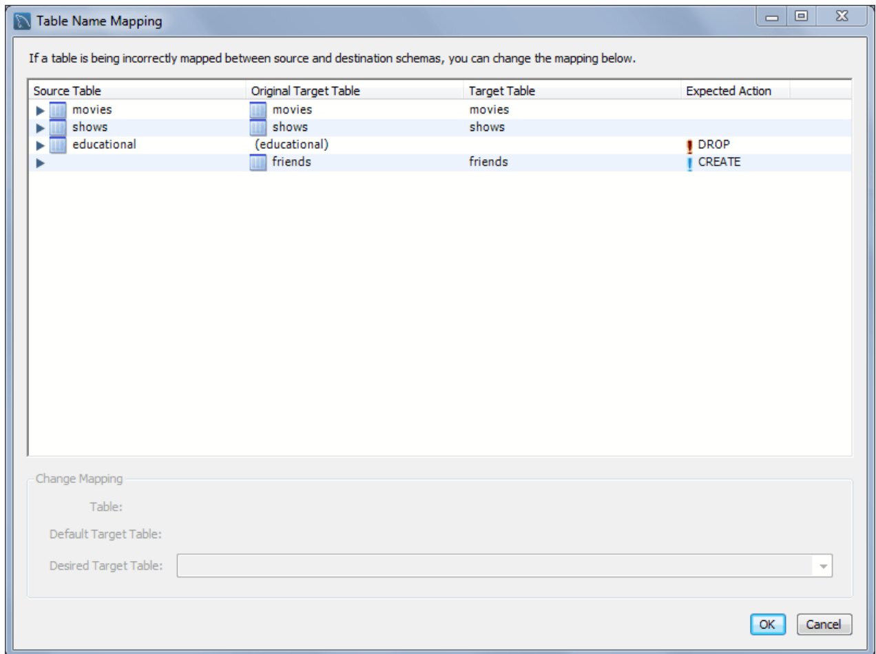
Figure 8.52 Table Mapping
