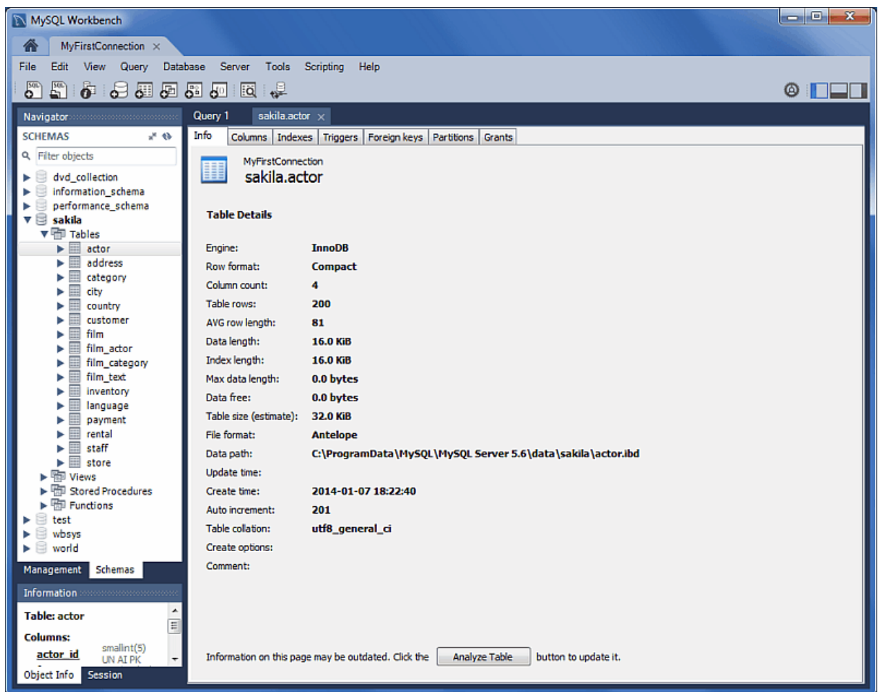
Figure 1.24 Table Inspector
