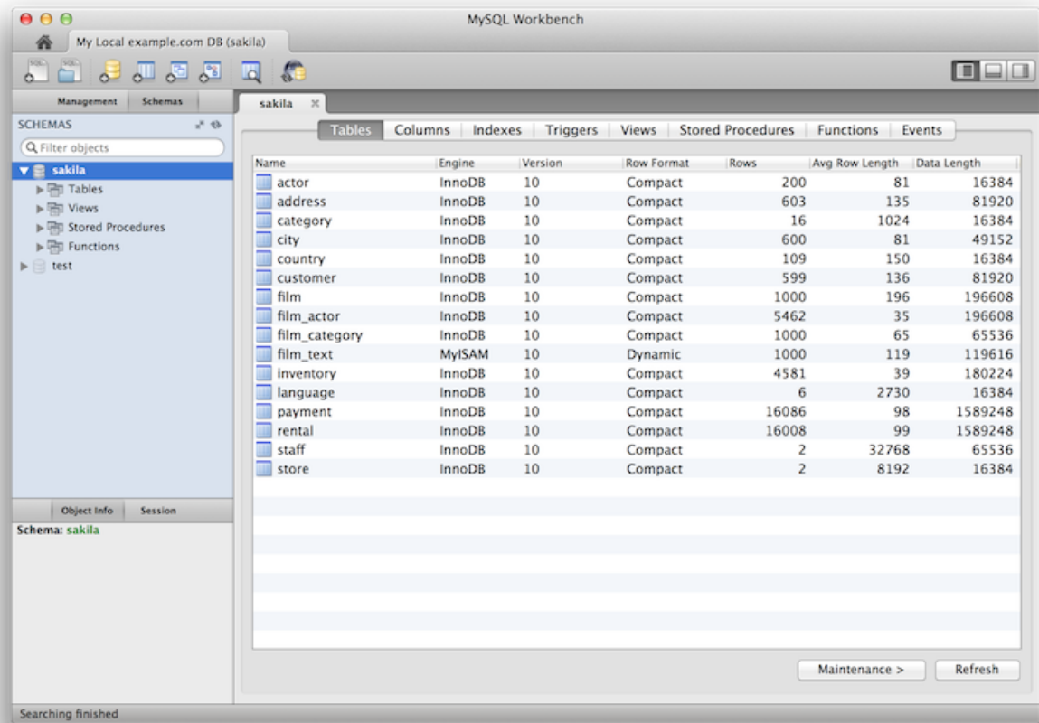
Figure 1.33 Schema Inspector
