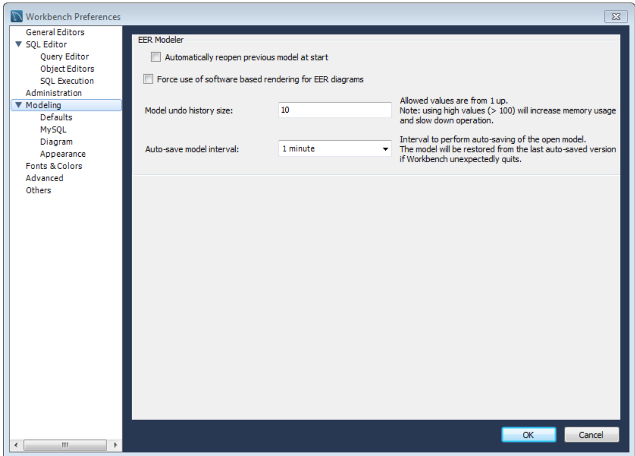
Figure 3.11 Preferences: Modeling
