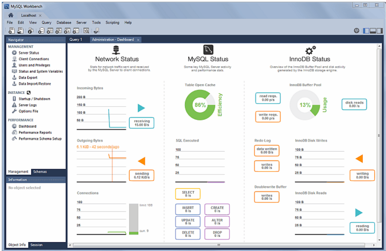
Figure 1.13 Performance Dashboard
