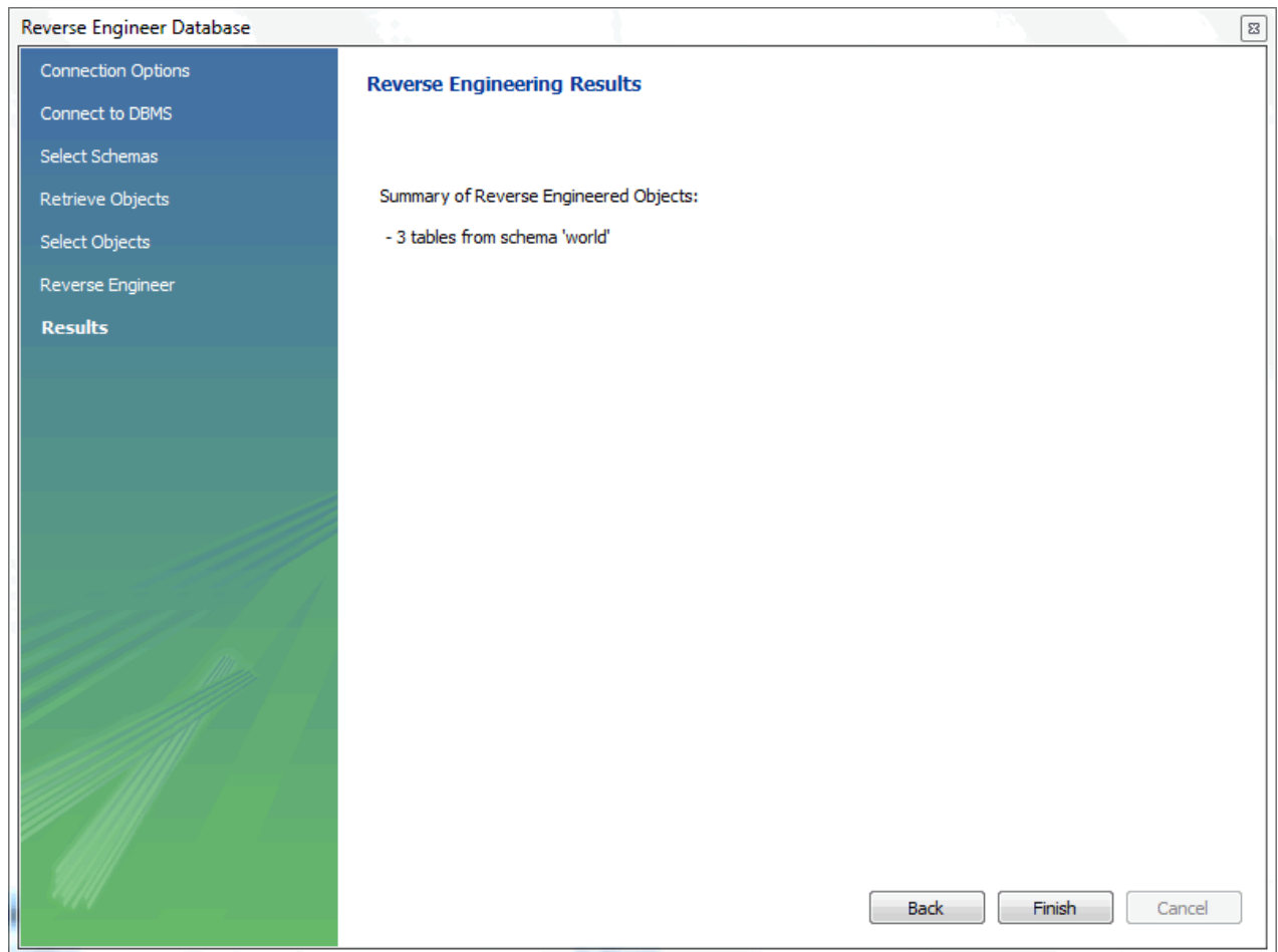
Figure 8.49 Results
