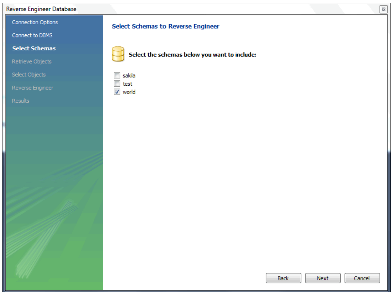
Figure 8.45 Select Schemas
