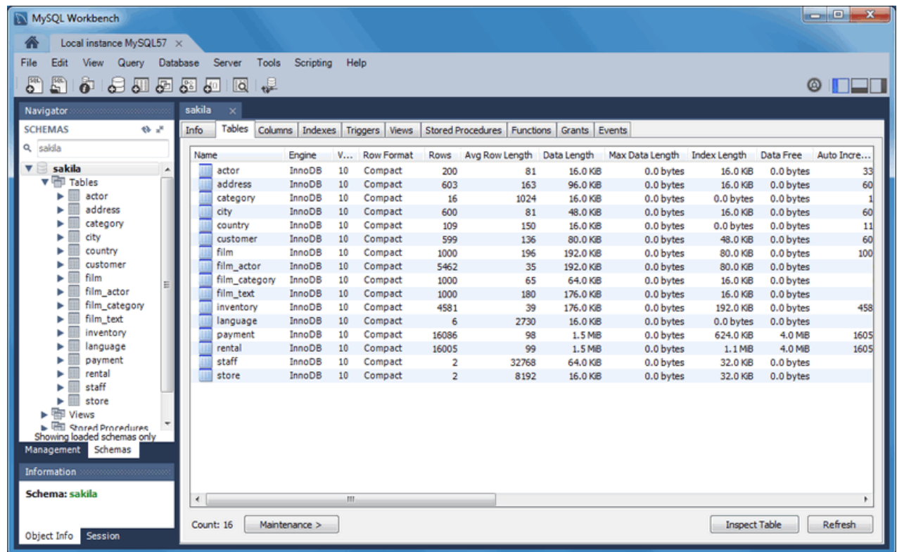
Figure 7.26 Schema Inspector
