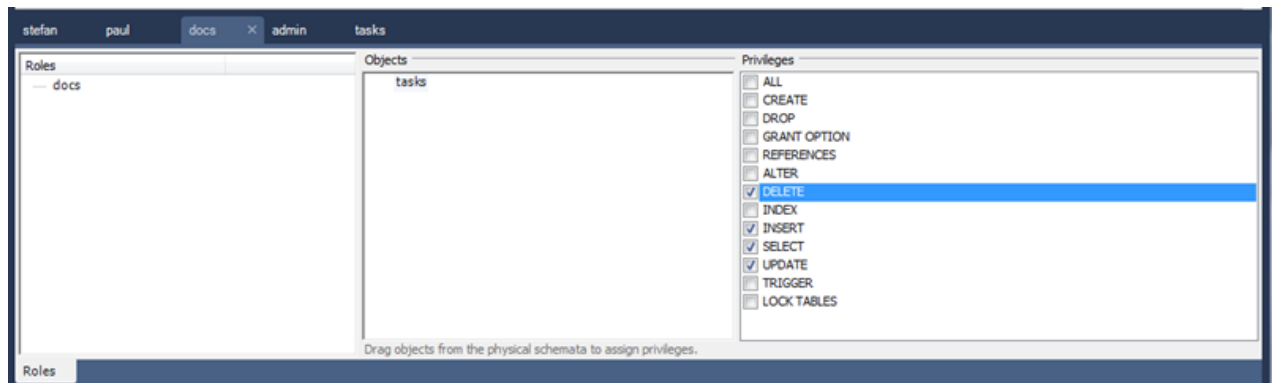
Figure 8.5 Role Editor
