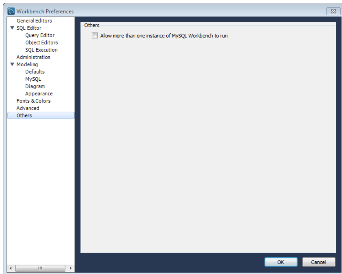
Figure 3.18 Preferences: Others
