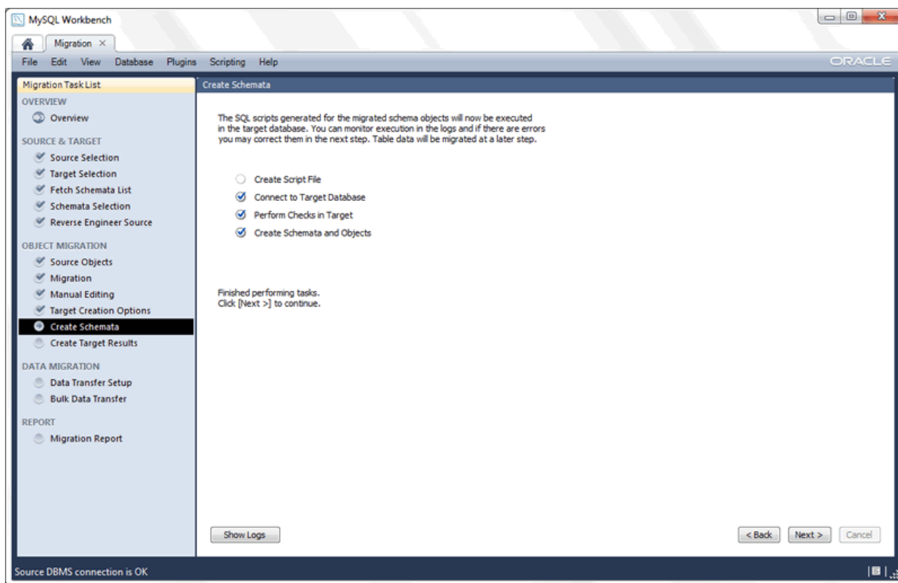
Figure 9.36 Create Schemata
