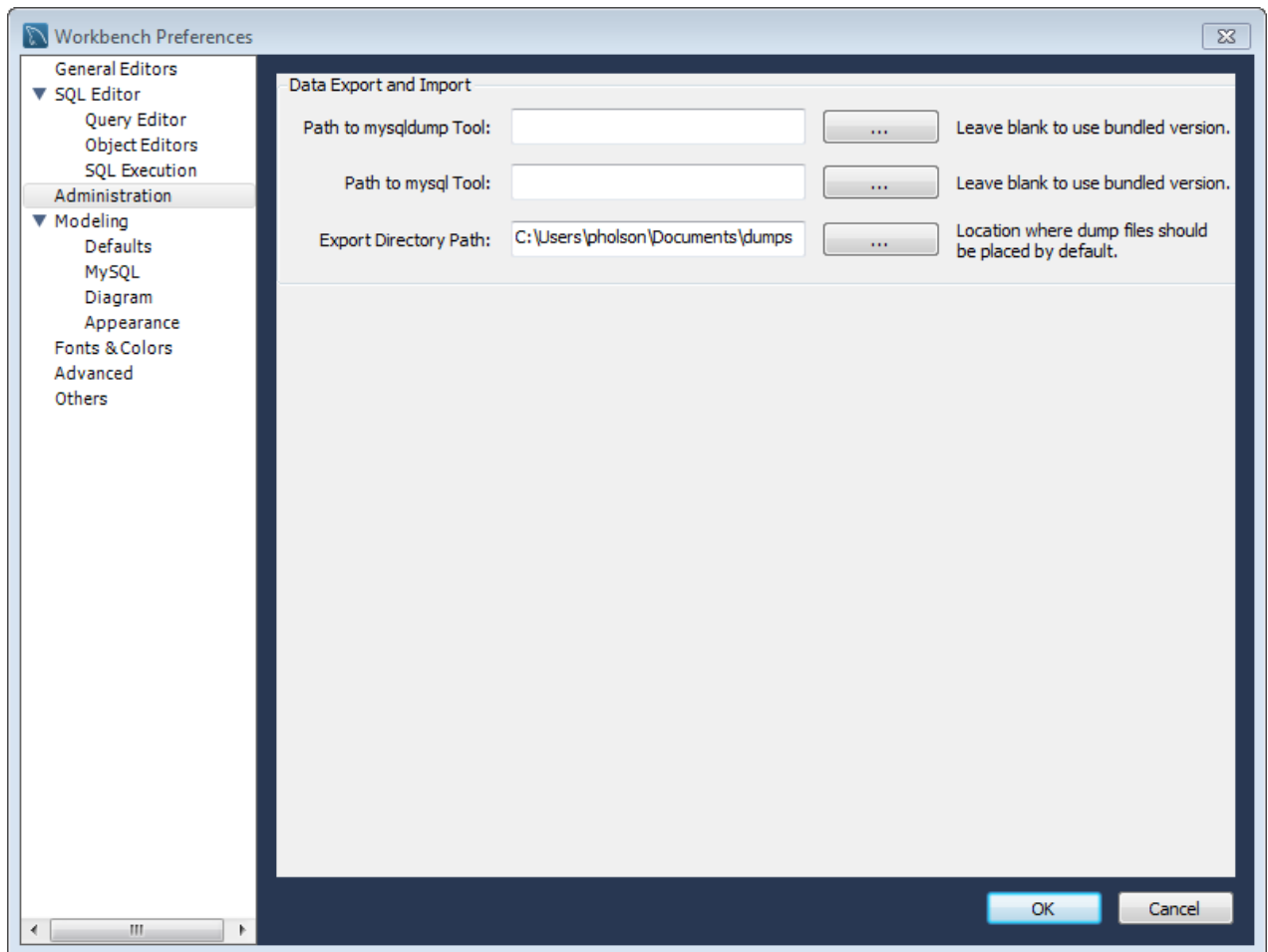
Figure 3.10 Preferences: Administration
