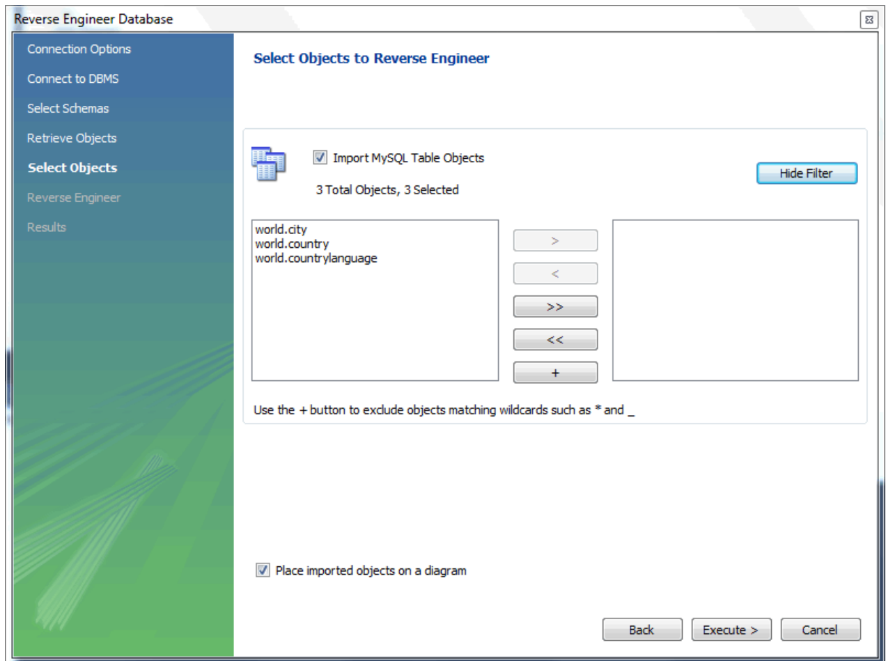
Figure 8.47 Select Objects
