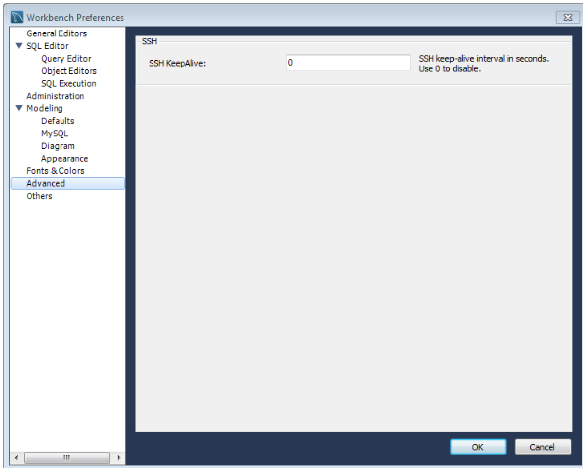
Figure 3.17 Preferences: Advanced
