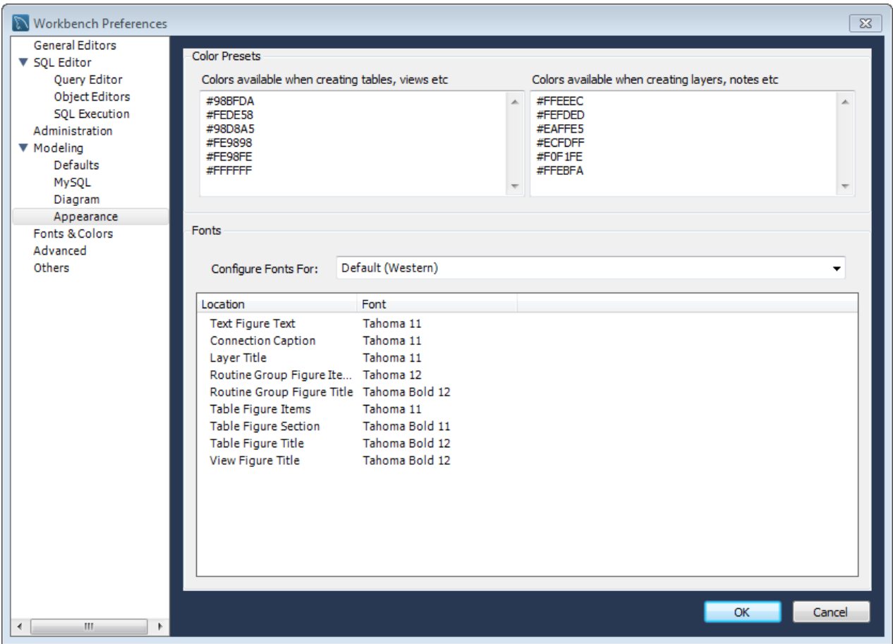
Figure 3.1 Appearance Preferences
