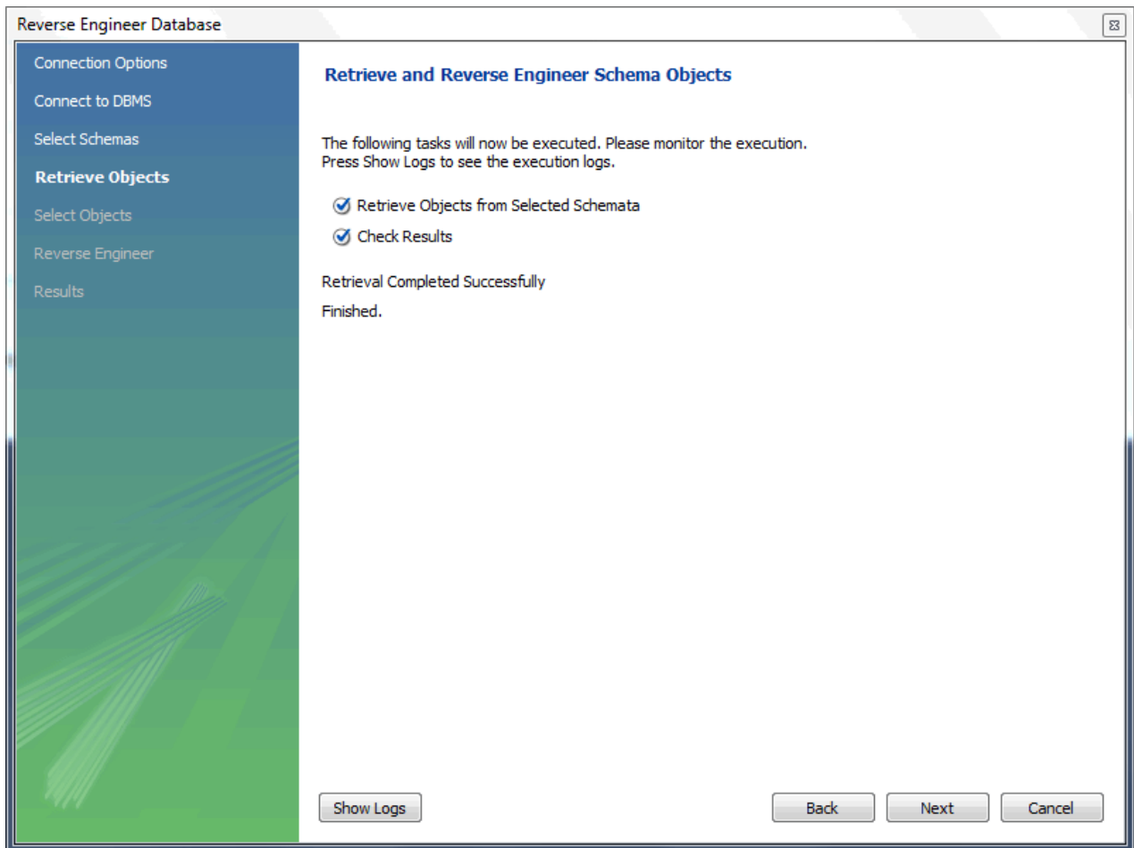
Figure 8.46 Retrieve Objects
