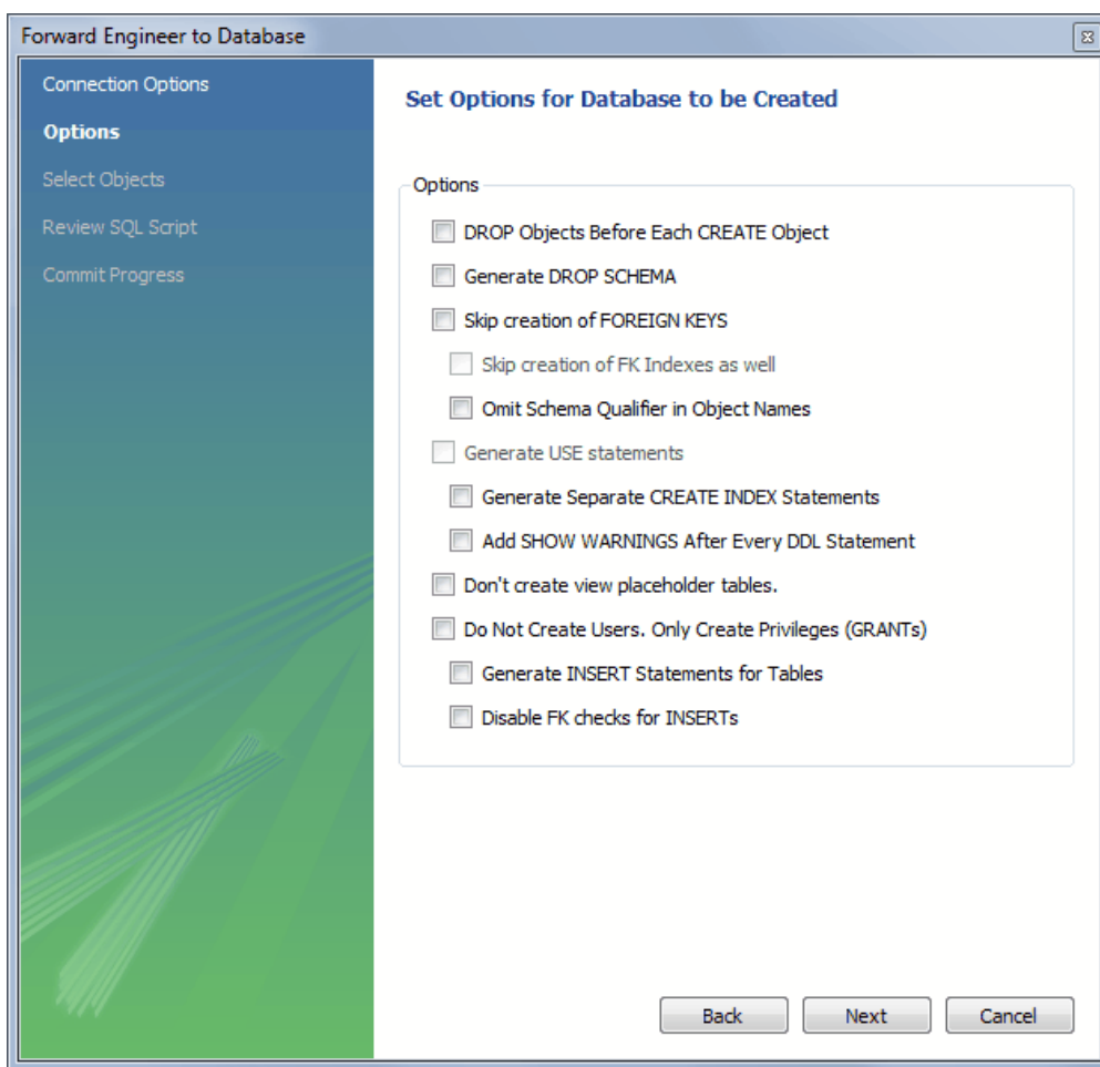
Figure 8.36 Options
