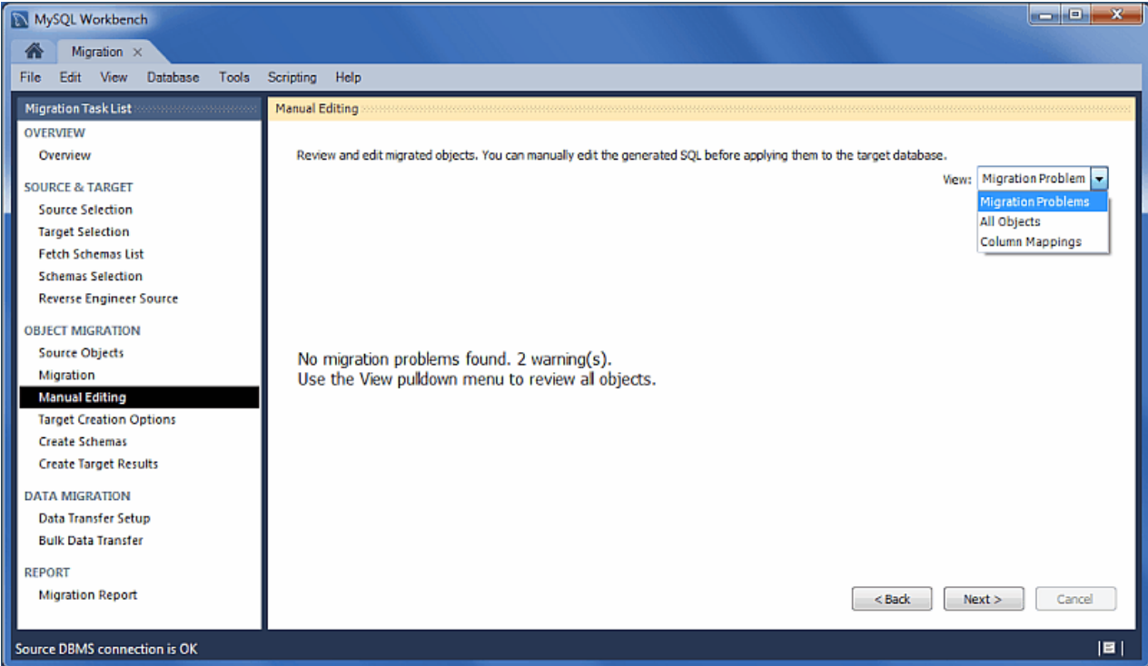
Figure 9.11 MySQL Workbench migration: Manual Editing (Migration Problems)
